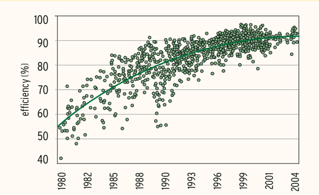
Efficiency factor of tested biomass boilers
