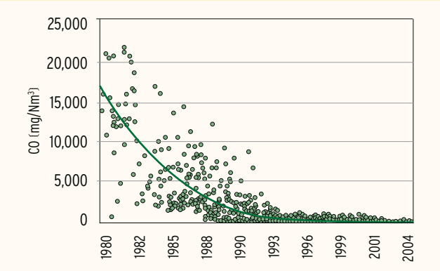
Carbon monoxide emissions of tested biomass boilers
